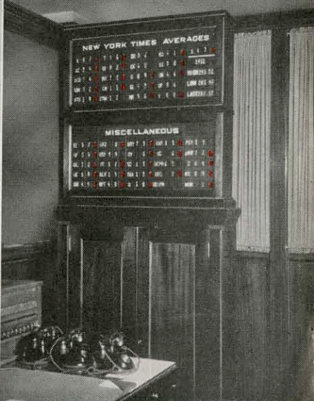
Executive Teleregisters display last prices. These units operate from a Main board.
